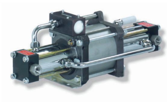
DLE 2 double acting, single air drive head single stage
