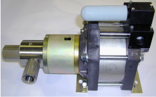
GSF15 (L) single acting, single air drive head with distance piece (Standard= Bottom inlet)
